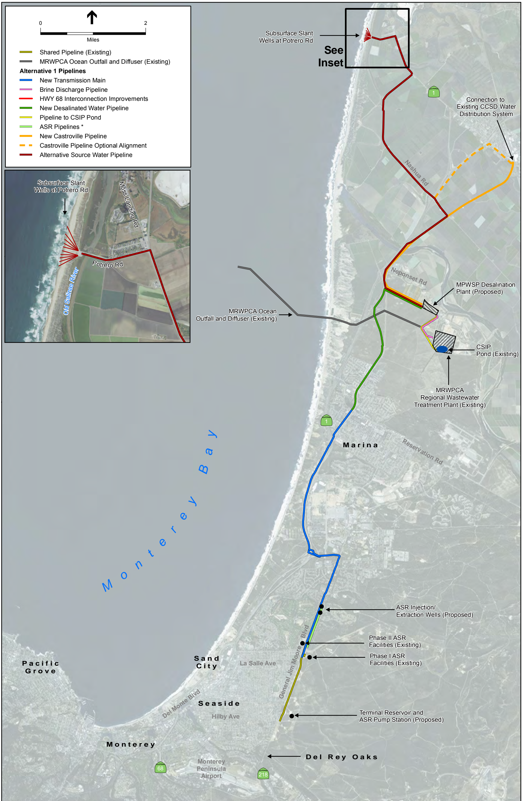
205335.01 Monterey Peninsula Water Supply Project Figure 5.4-1 Alternative 1- Slant Wells at Potrero Road
