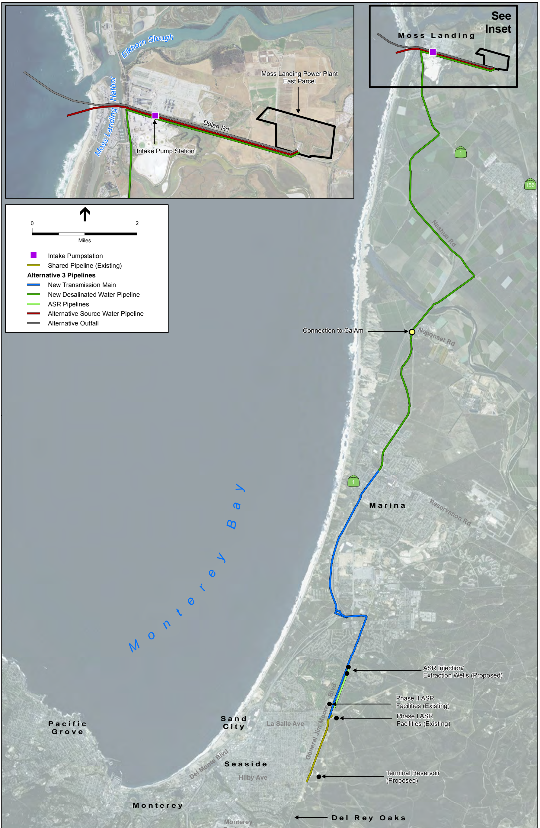
205335.01 Monterey Peninsula Water Supply Project Figure 5.4-3 Alternative 3 - Monterey Bay Regional Water Project
