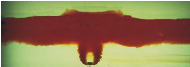
Figure 14. Trapped buoyant plume from multiport diffuser in stratified environment, from Roberts et al. (1989).
