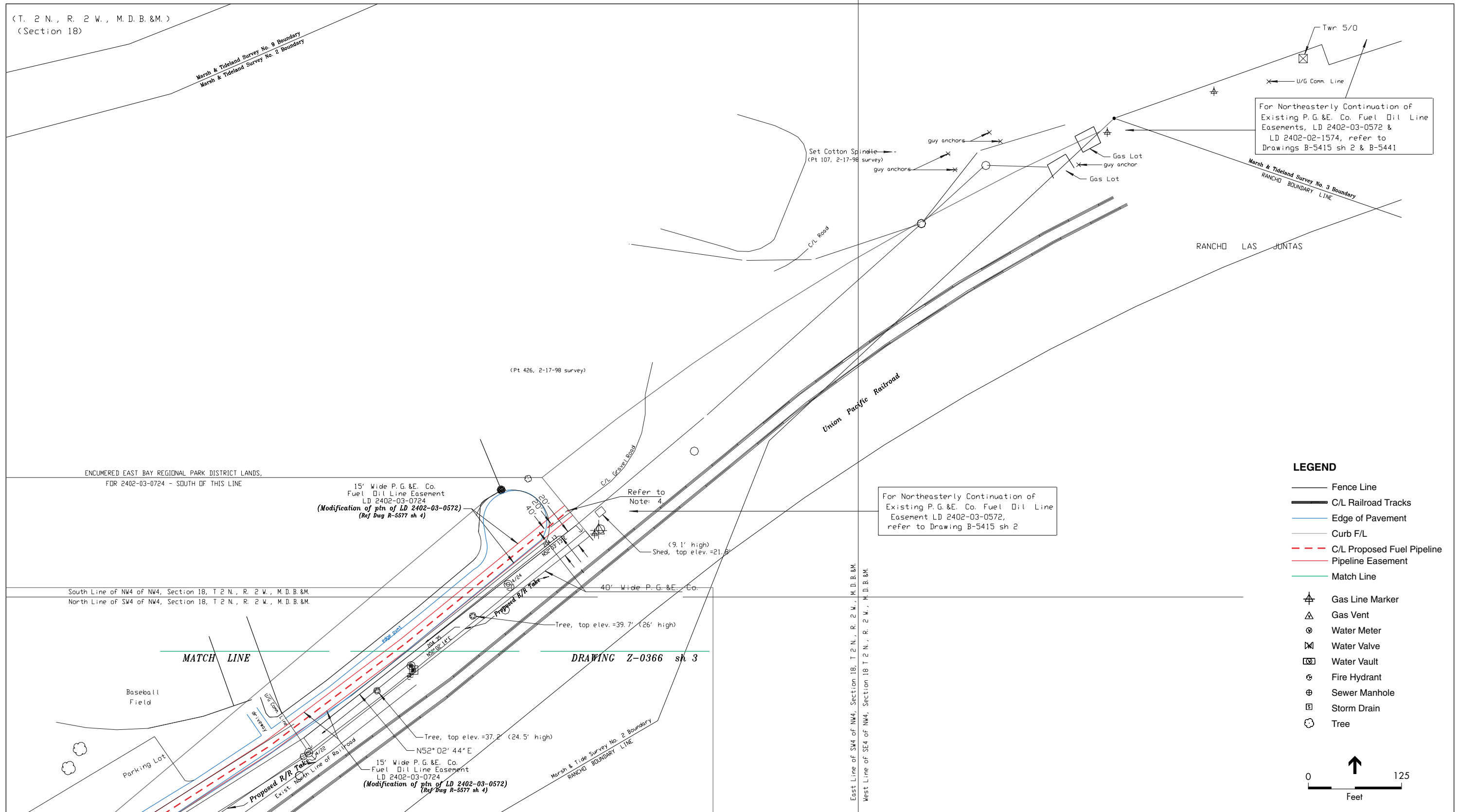
Figure 1-6 Proposed 4000' Replacement Pipeline (Drawing Z-0366 Sheet 4)
