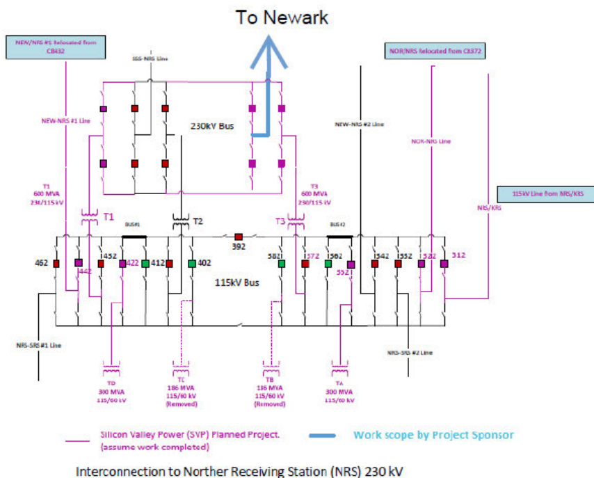
NRS 230 kV Substation
