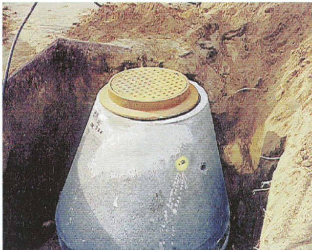
Manhole Installation
