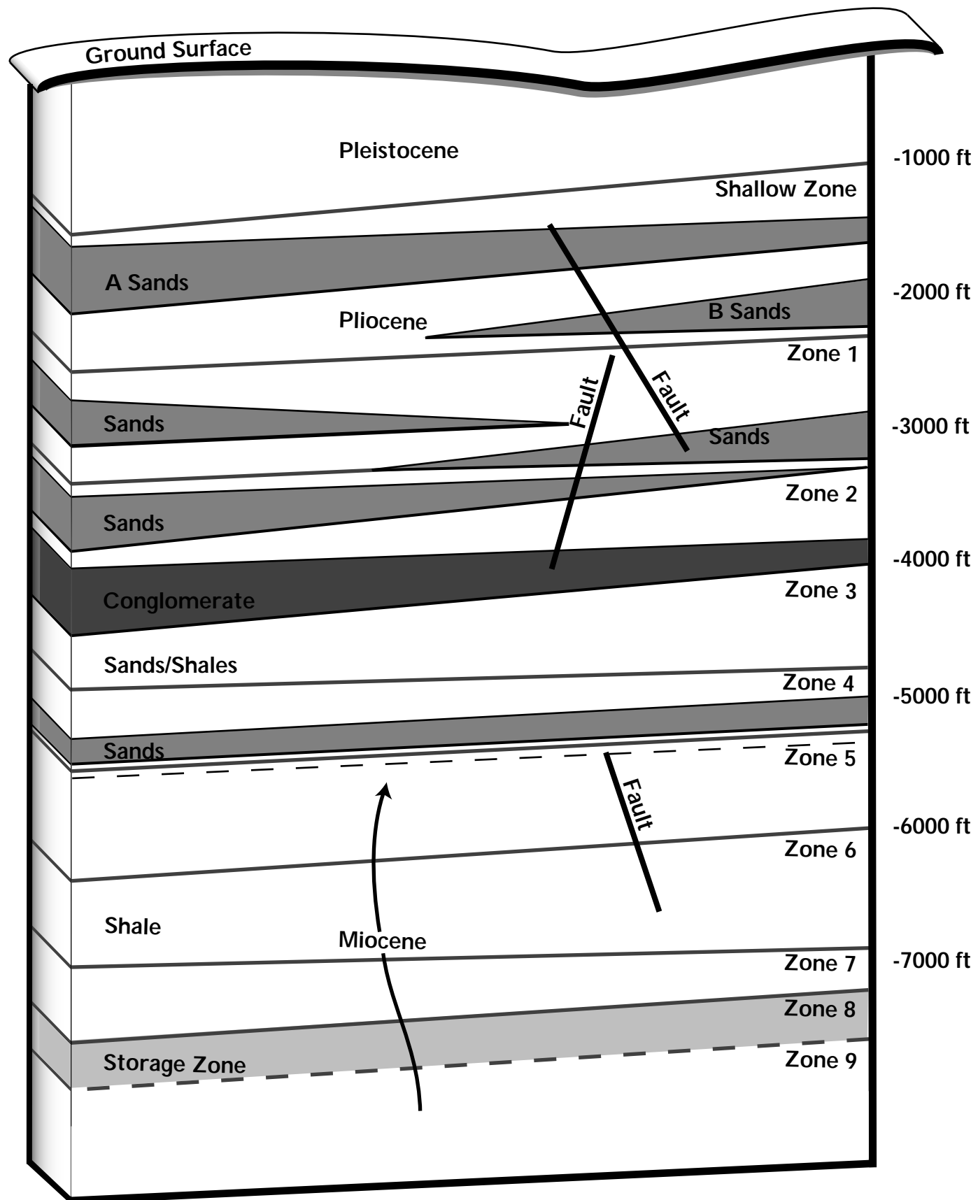
Figure 4.6-2: Subsurface Geologic Cross-Section
