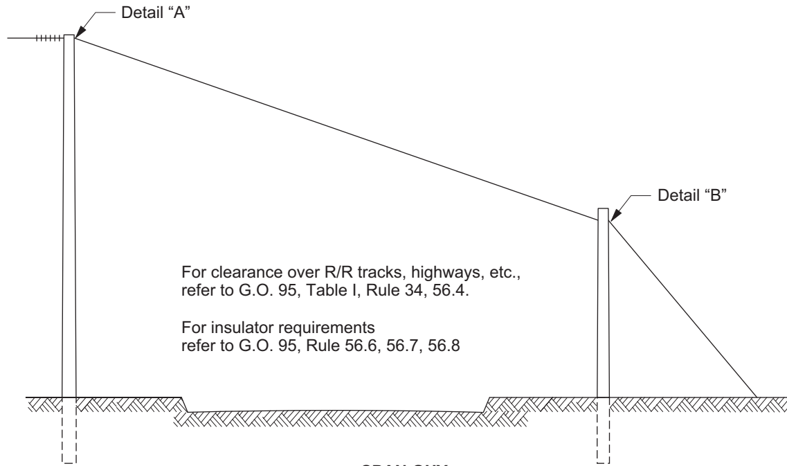
Figure 217-1: Span Guy Assemblies
