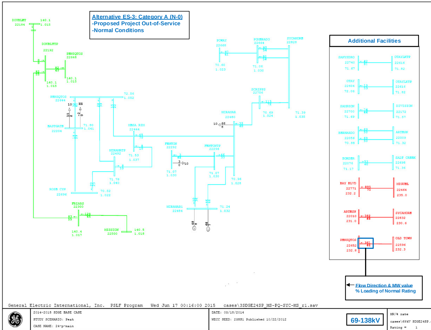
Figure 12 – ES-3, 69/138 kV Power Flow Plot, Normal conditions
