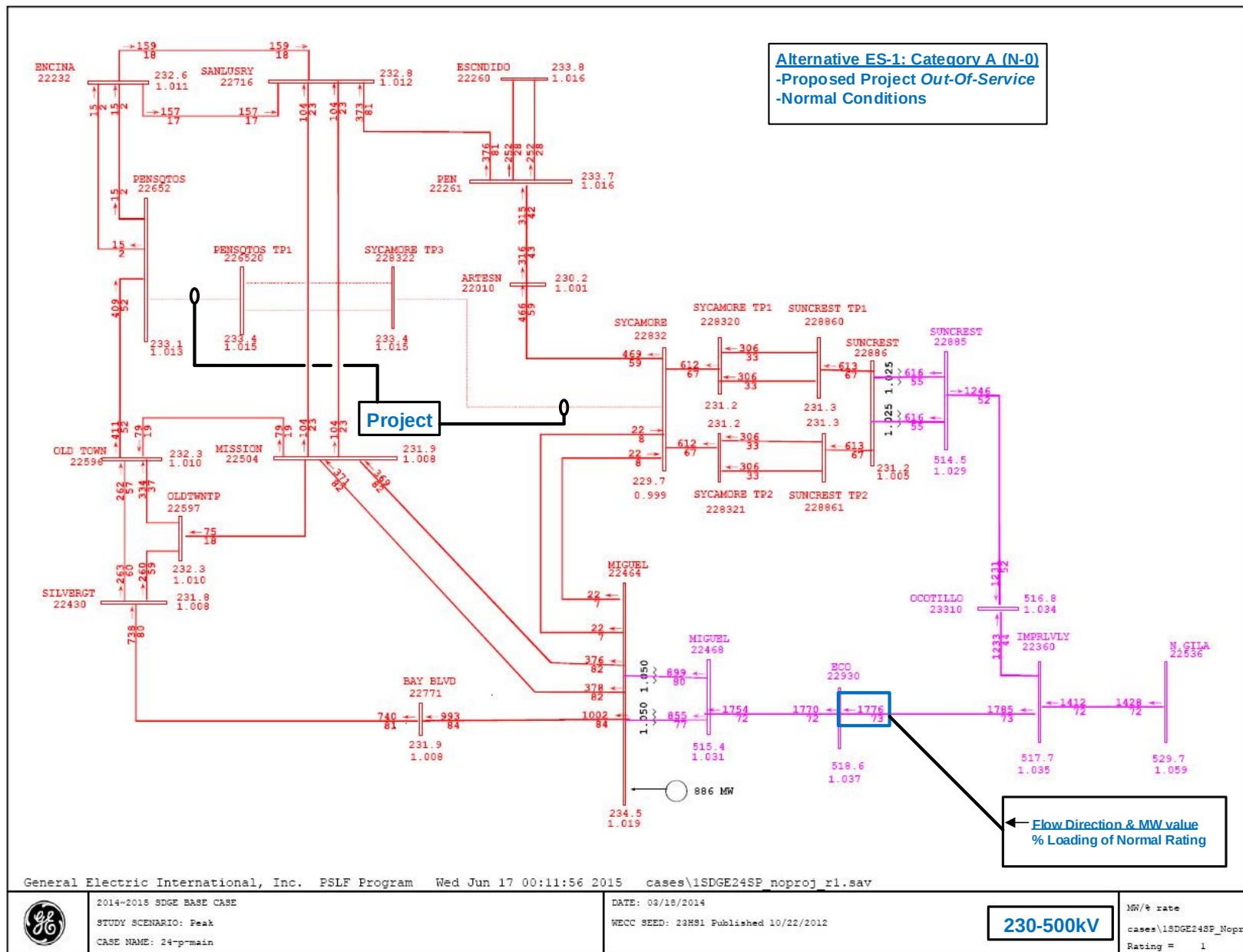
Figure 4 - ES-1, 230/500 kV Power Flow Plot, Normal condition
