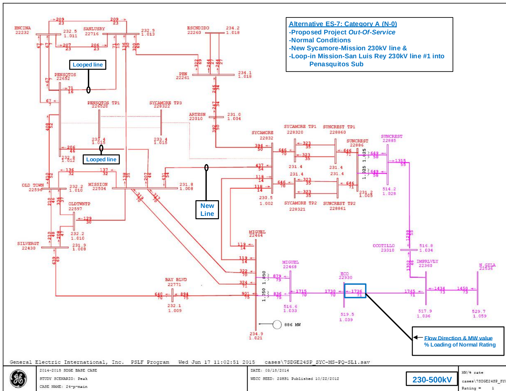
Figure 21 – ES-7, 230/500 kV Power Flow Plot, Normal conditions
