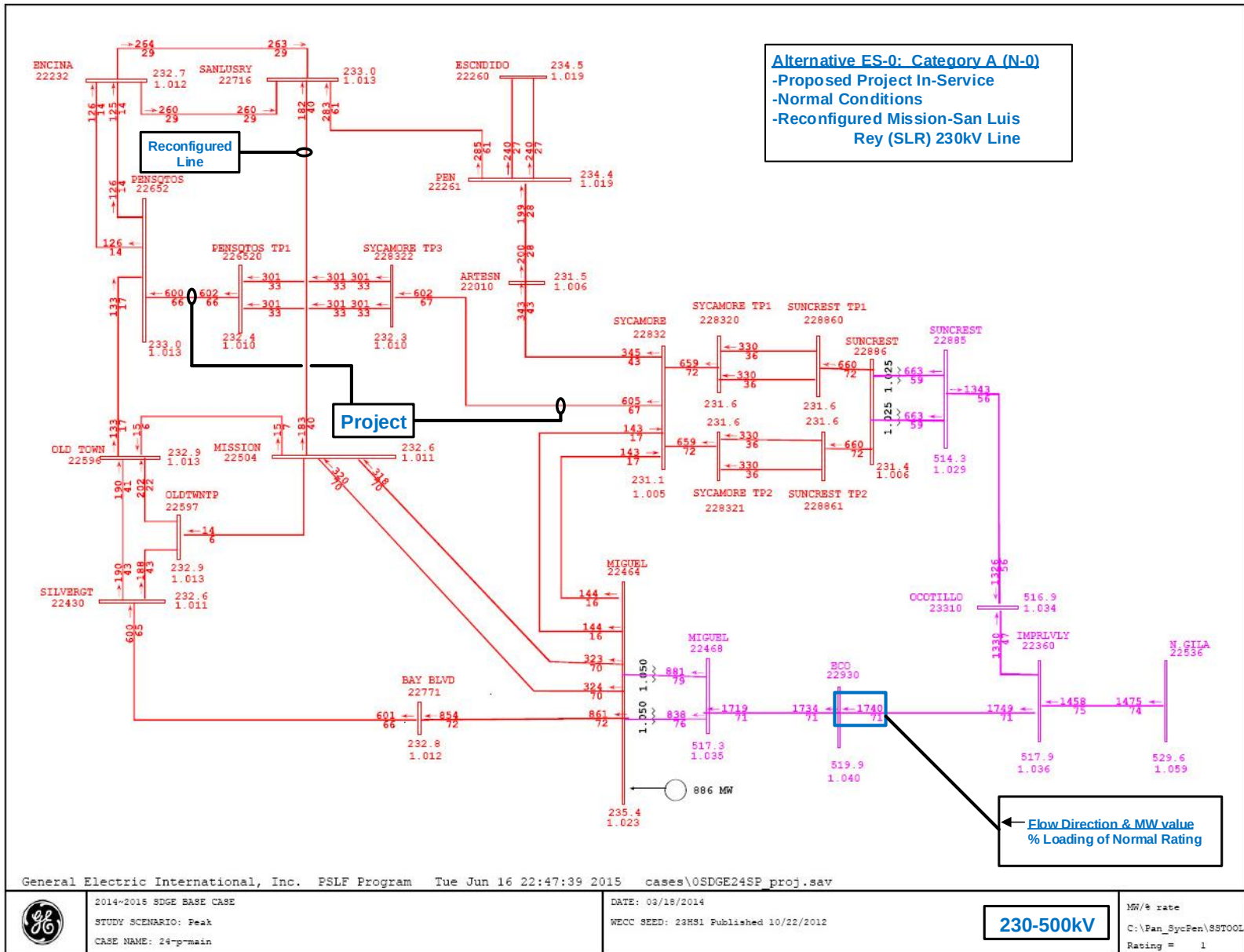
Figure 1 – ES-0, Proposed Project Power Flow Plot under Normal conditions
