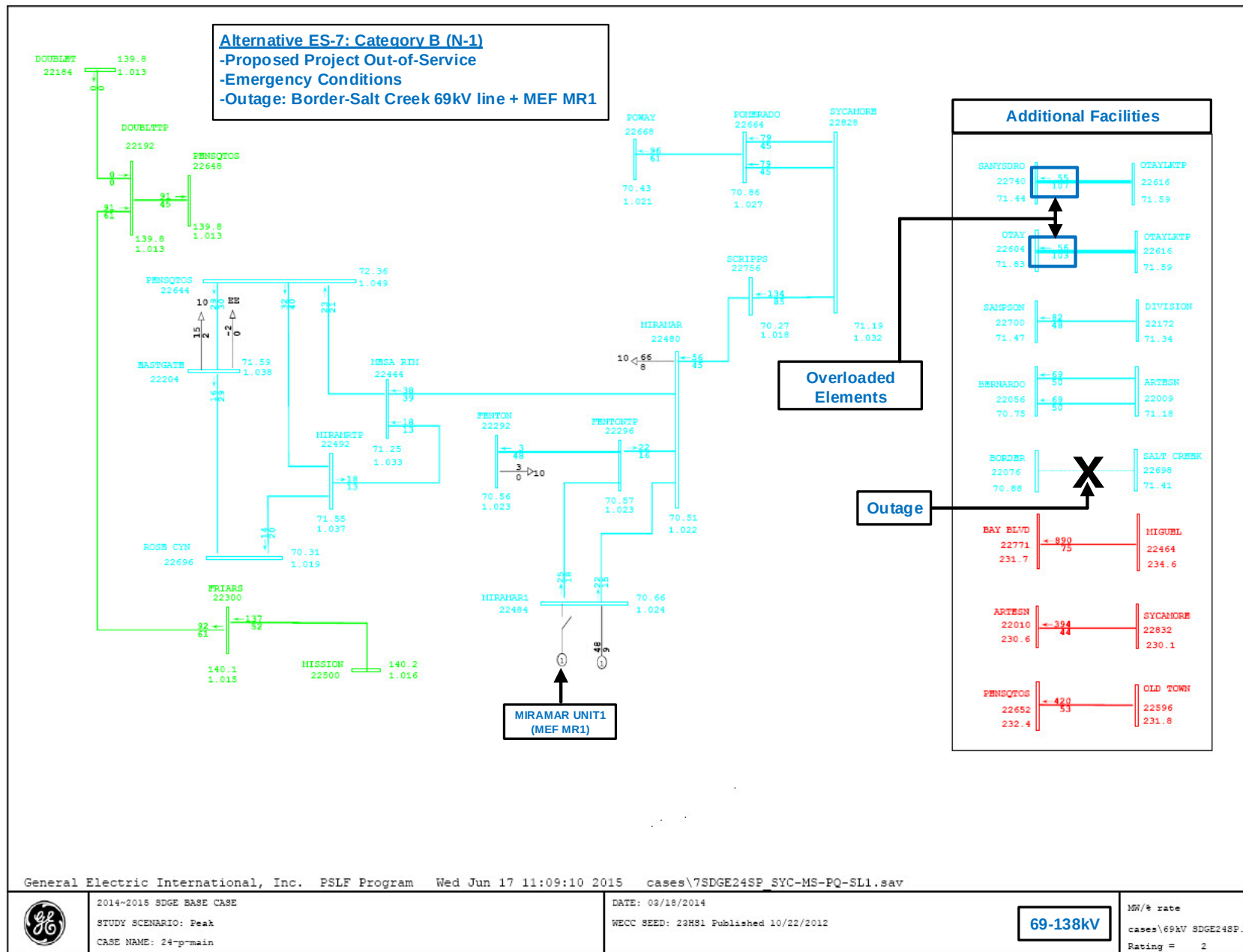
Figure 23 – ES-7, 69/138 kV Power Flow Plot, Single contingency
