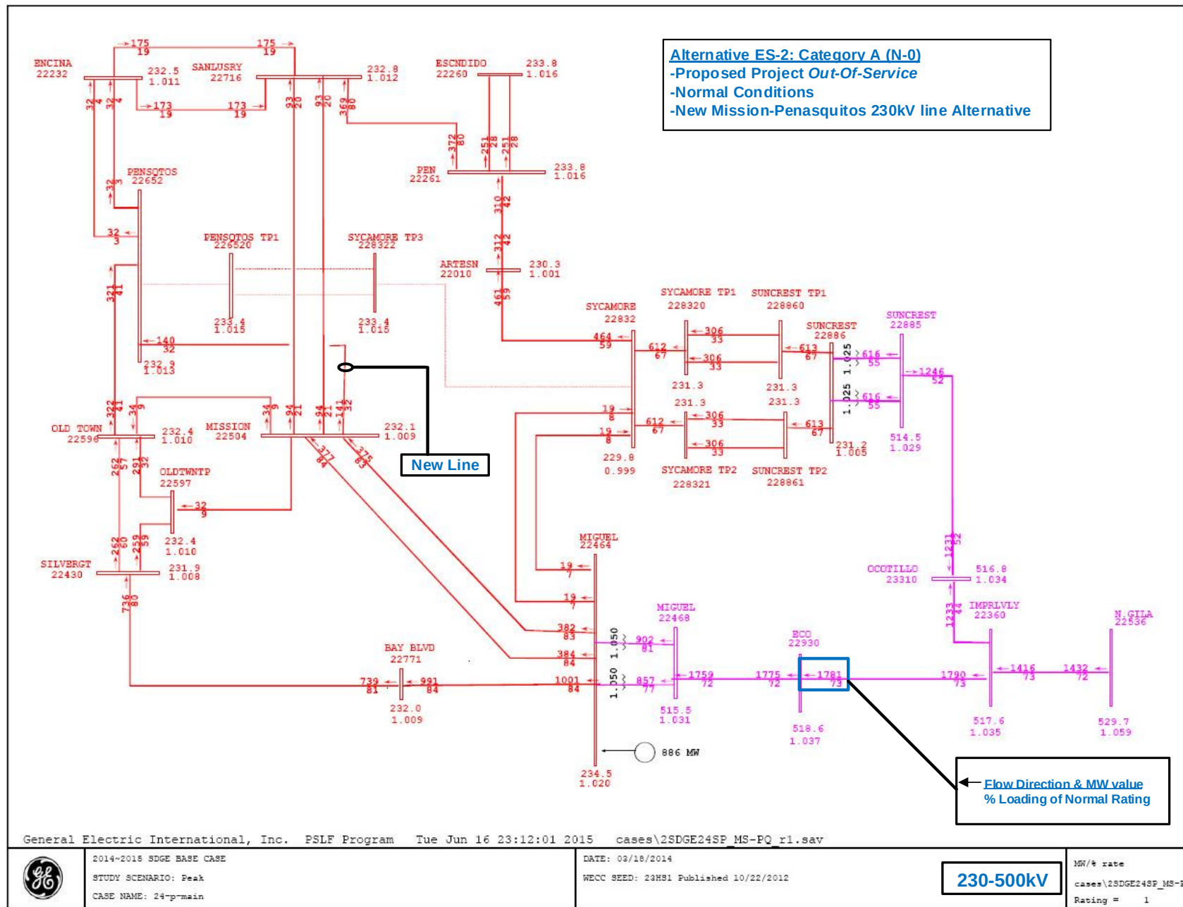
Figure 7 – ES-2, 230/500 kV Power Flow Plot, Normal conditions
