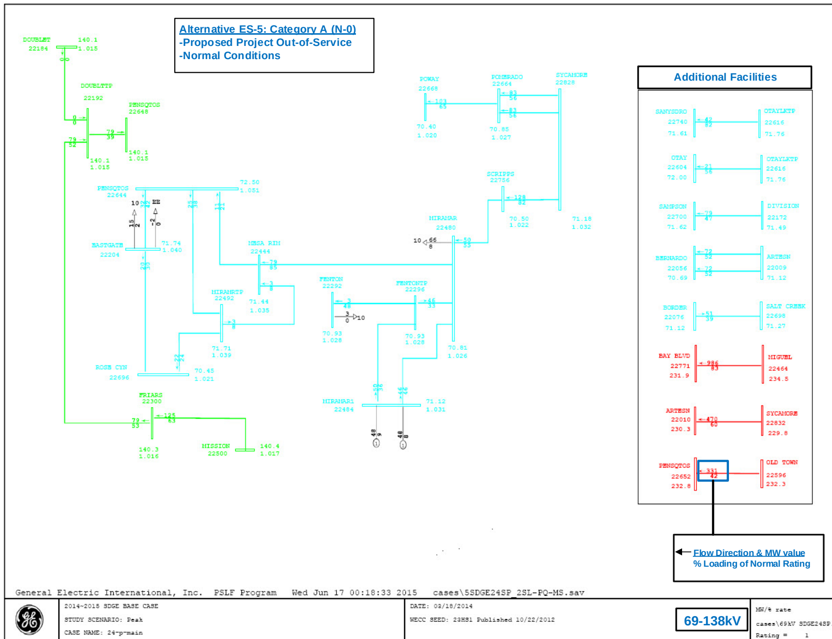
Figure 17 – ES-5, 69/138 kV Power Flow Plot, Normal condition
