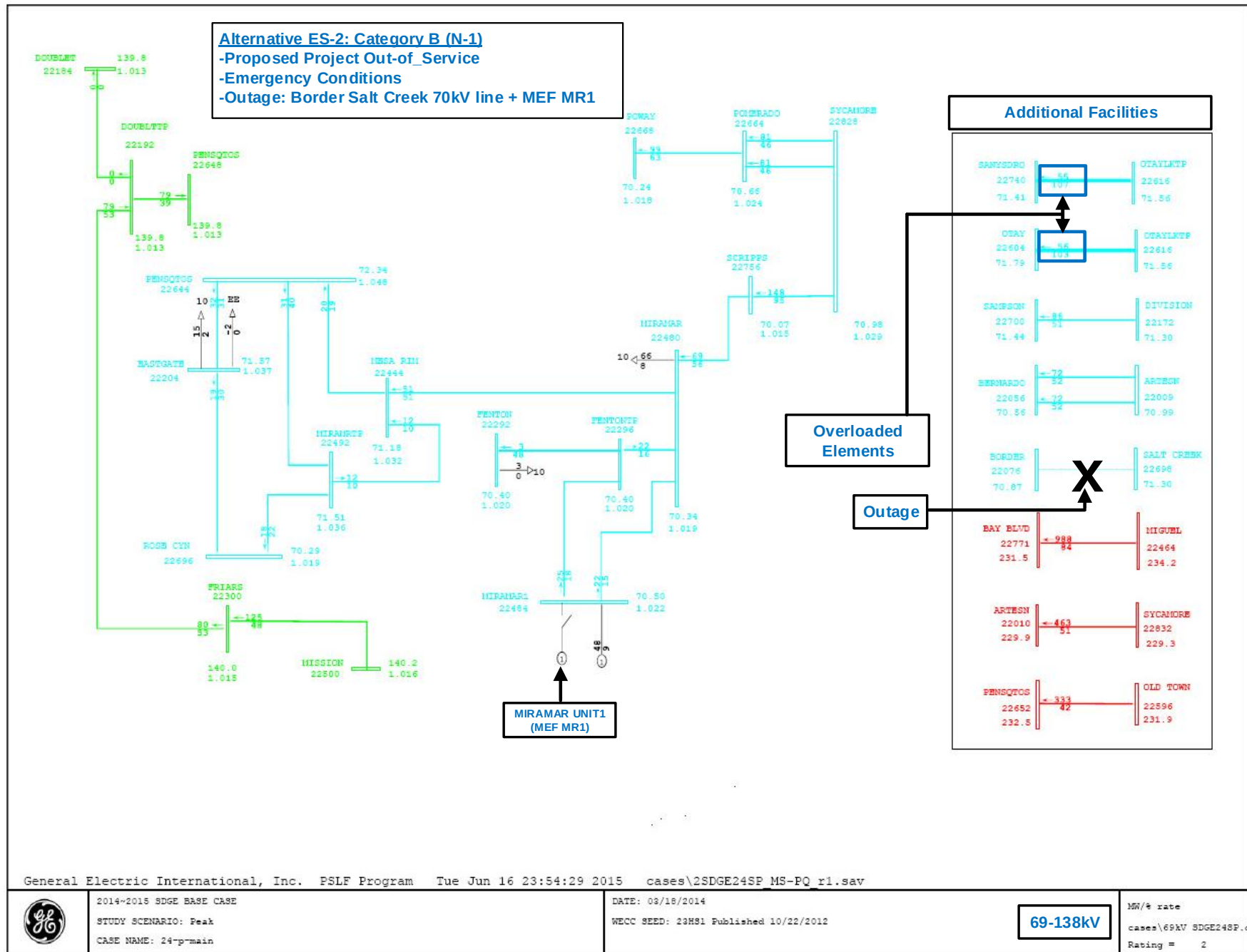
Figure 10 – ES-2, 69/138 kV Power Flow Plot, Single contingency
