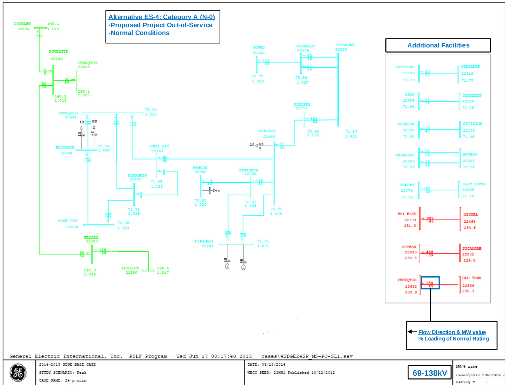
Figure 15 – ES-4, 69/138 kV Power Flow Plot, Normal conditions
