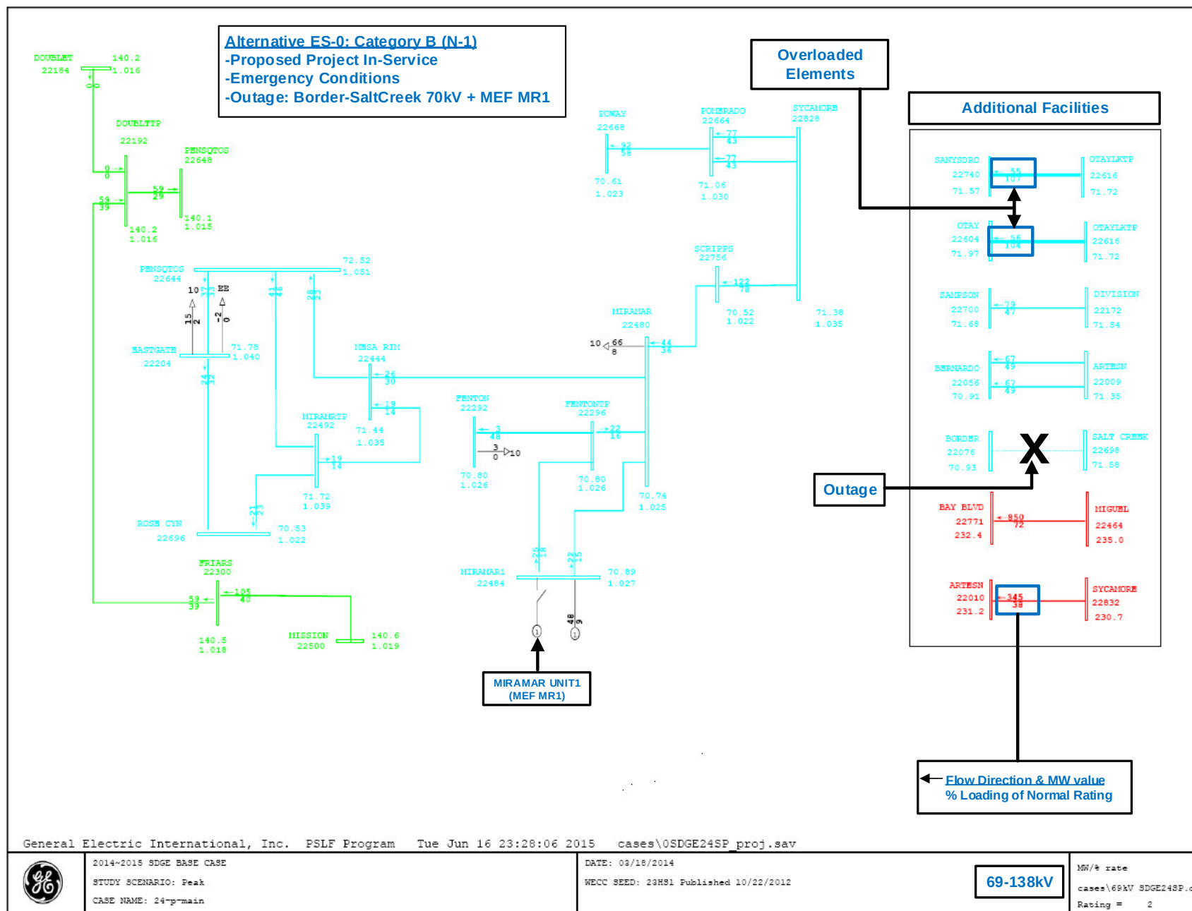
Figure 3 - ES-0, Power Flow Plot for Category B contingencies (69/138 kV System)
