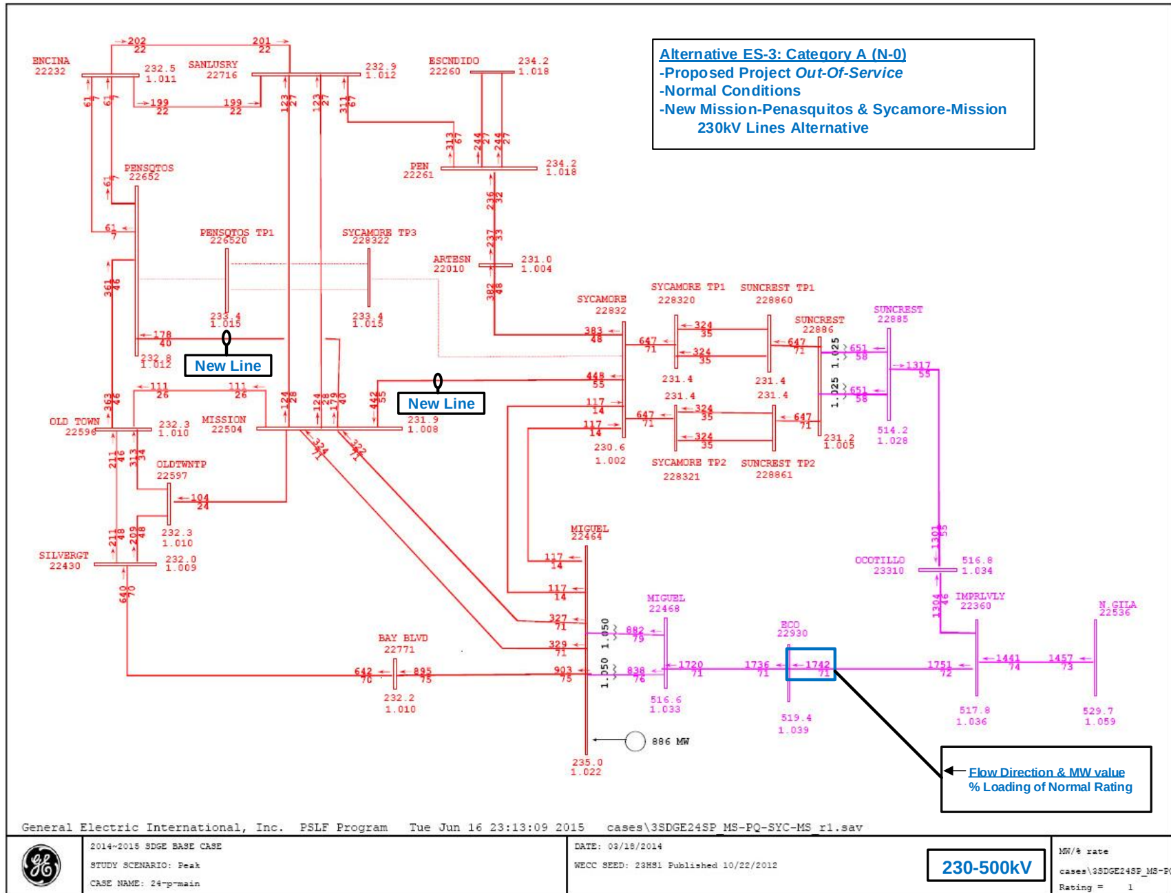
Figure 11 – ES-3, 230/500 kV Power Flow Plot, Normal conditions
