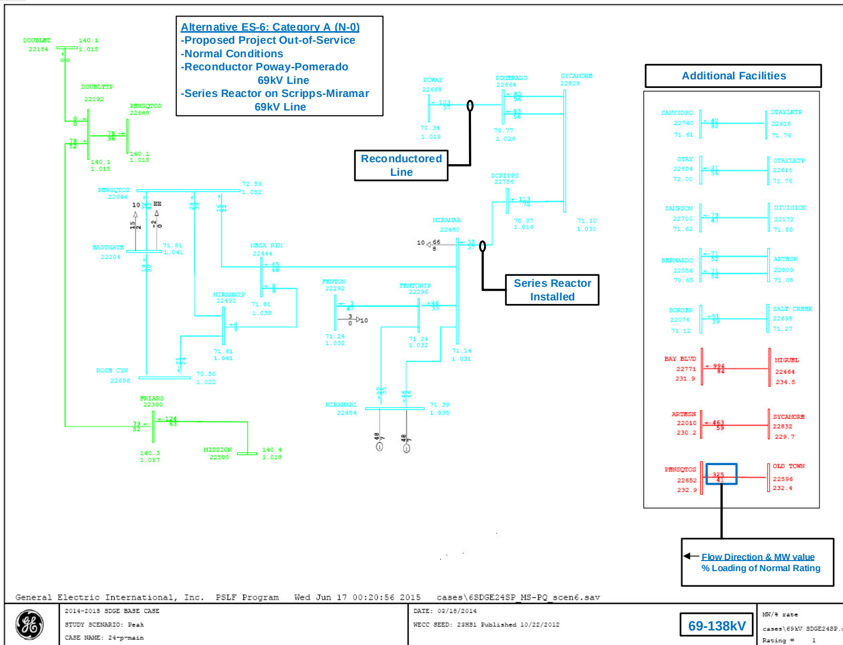
Figure 19 – ES-6, 69/138 kV Power Flow Plot, Normal condition
