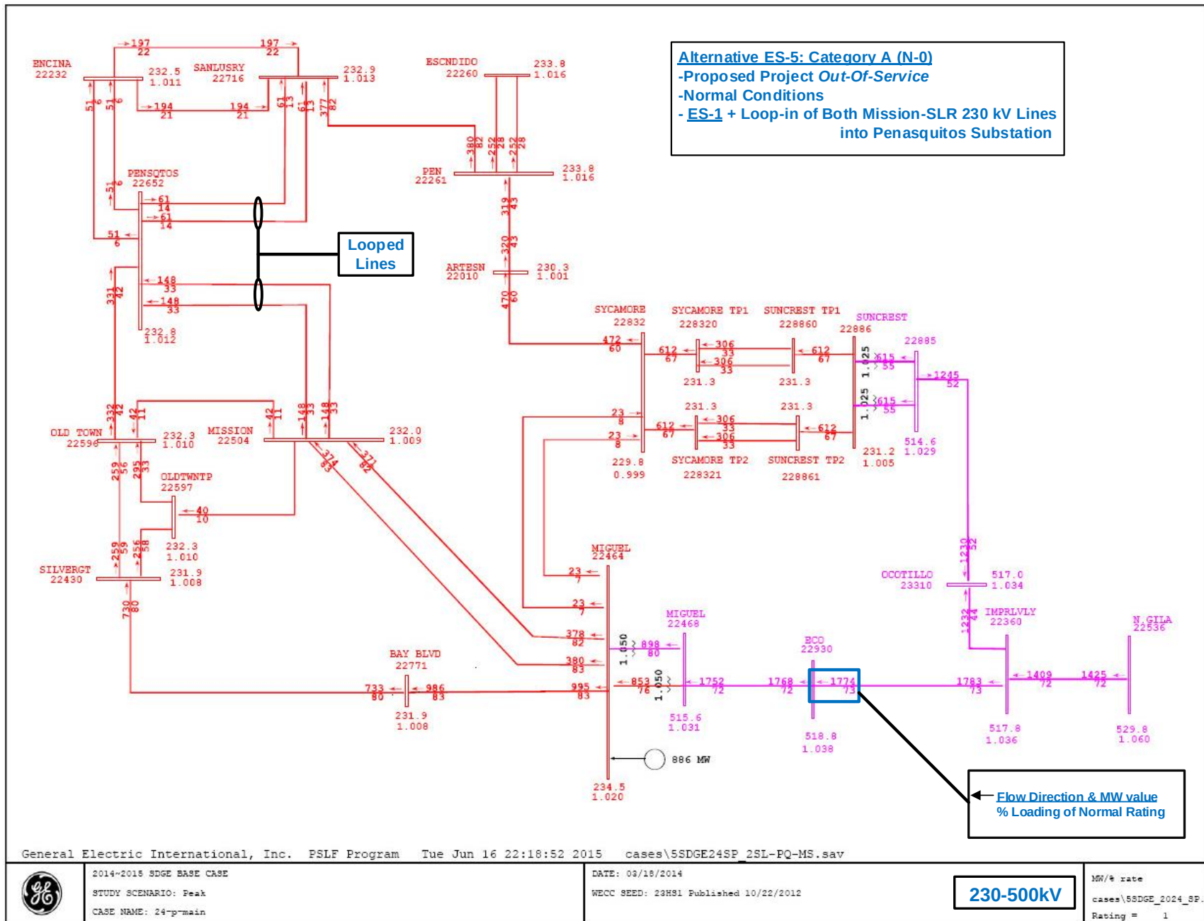
Figure 16 – ES-5, 230/500 kV Power Flow Plot, Normal condition
