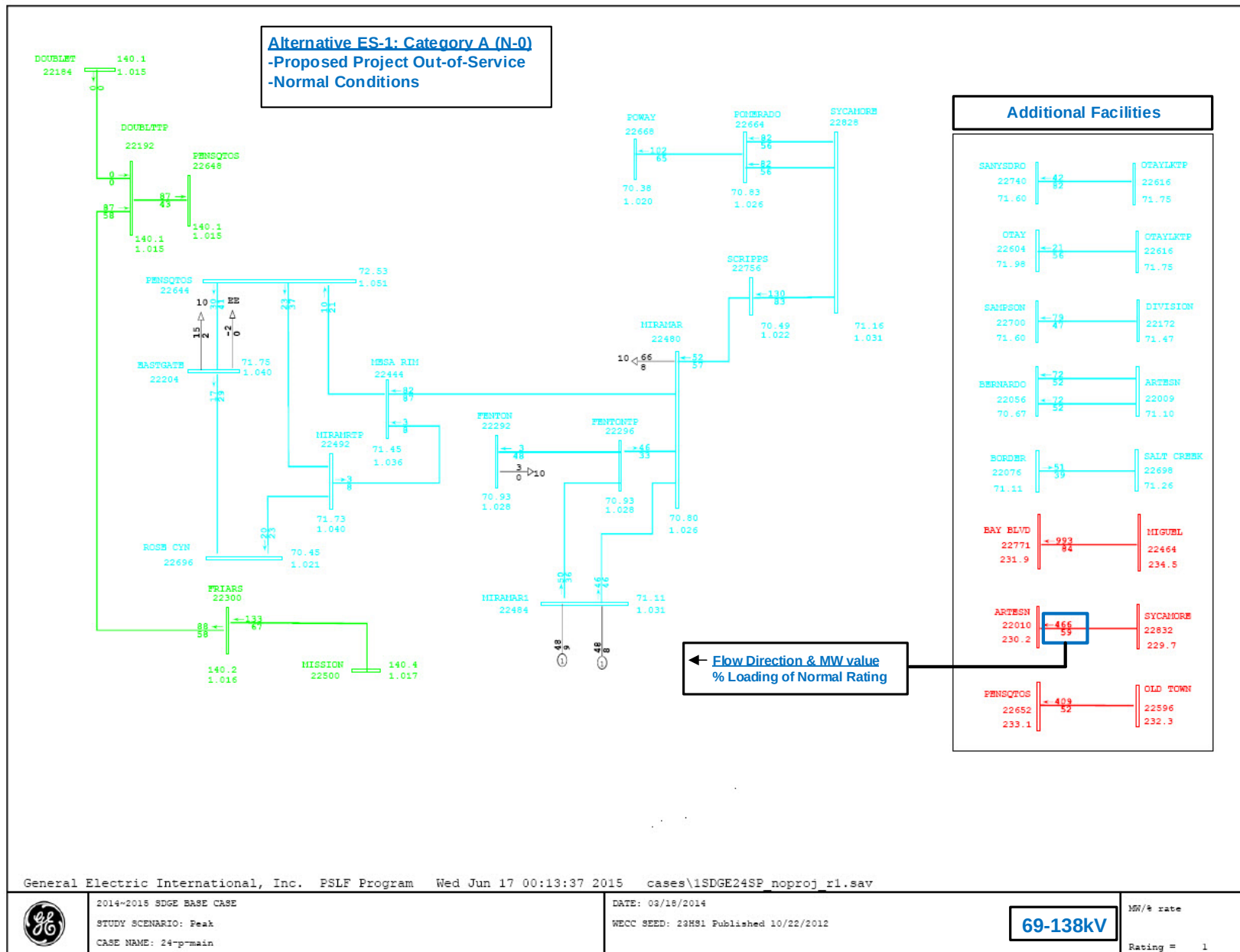
Figure 5 - ES-1, 69/138 kV Power Flow Plot, Normal condition
