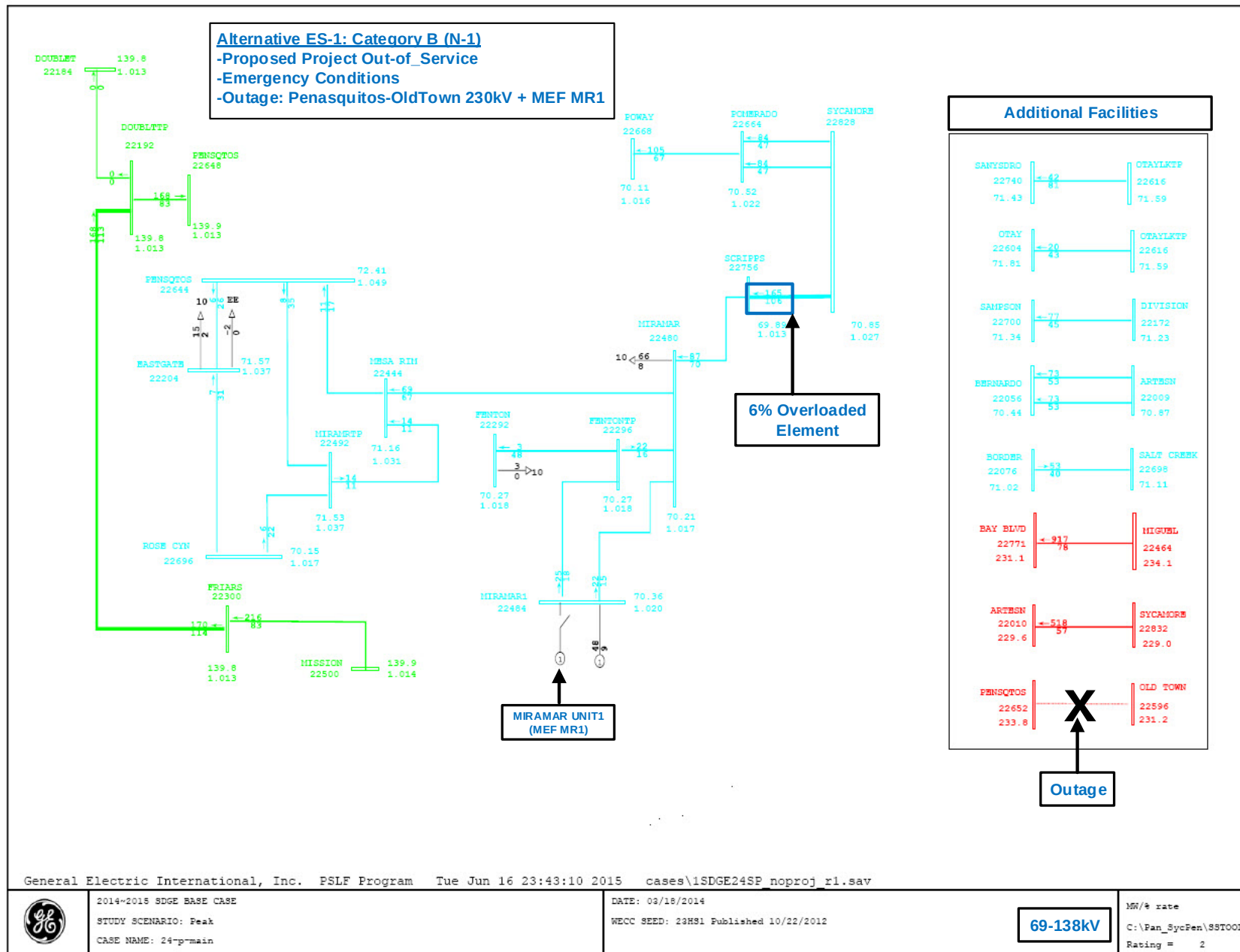
Figure 6 - ES-1, 69/138 kV Power Flow Plot, Single contingency condition
