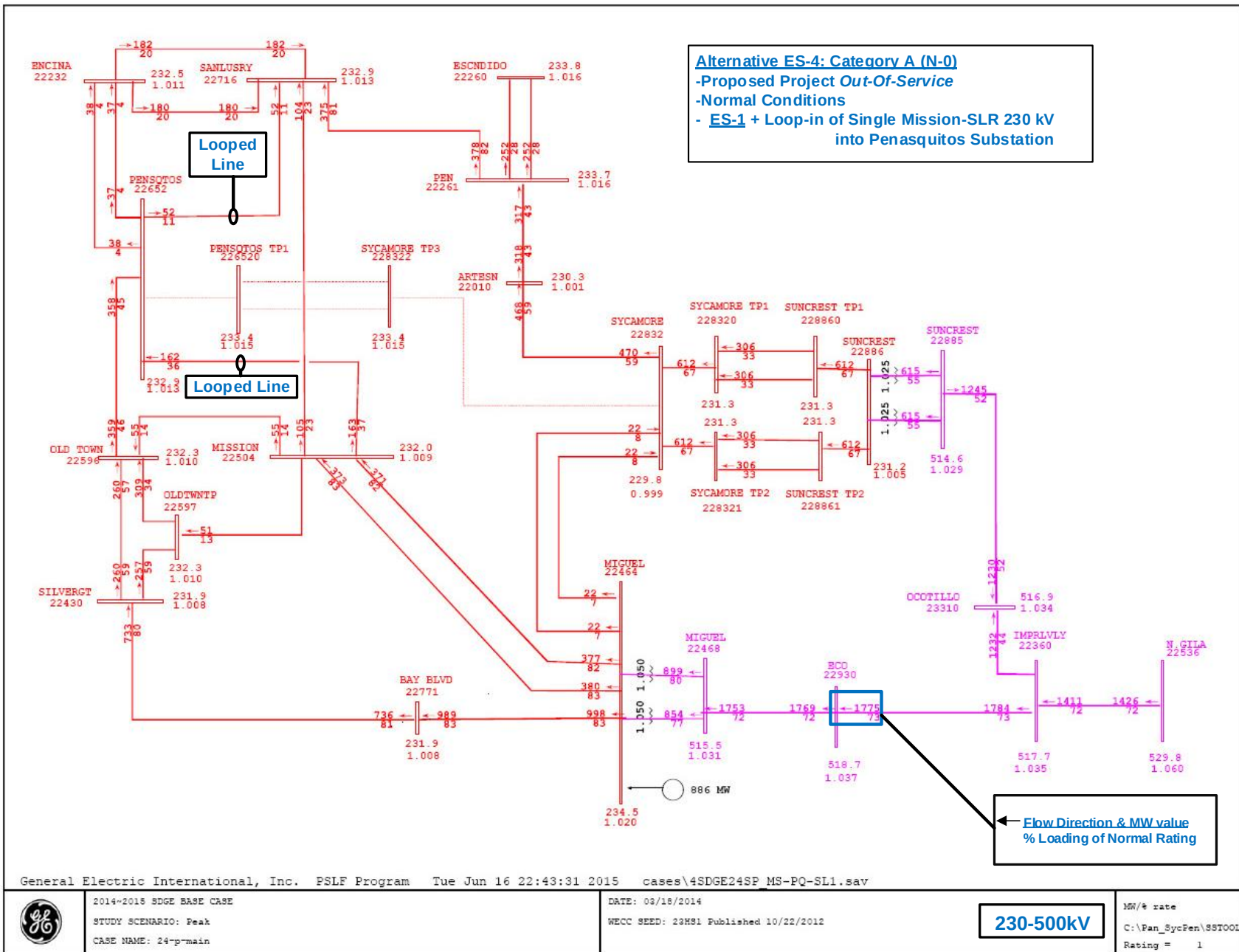
Figure 14 – ES-4, 230/500 kV Power Flow Plot, Normal conditions
