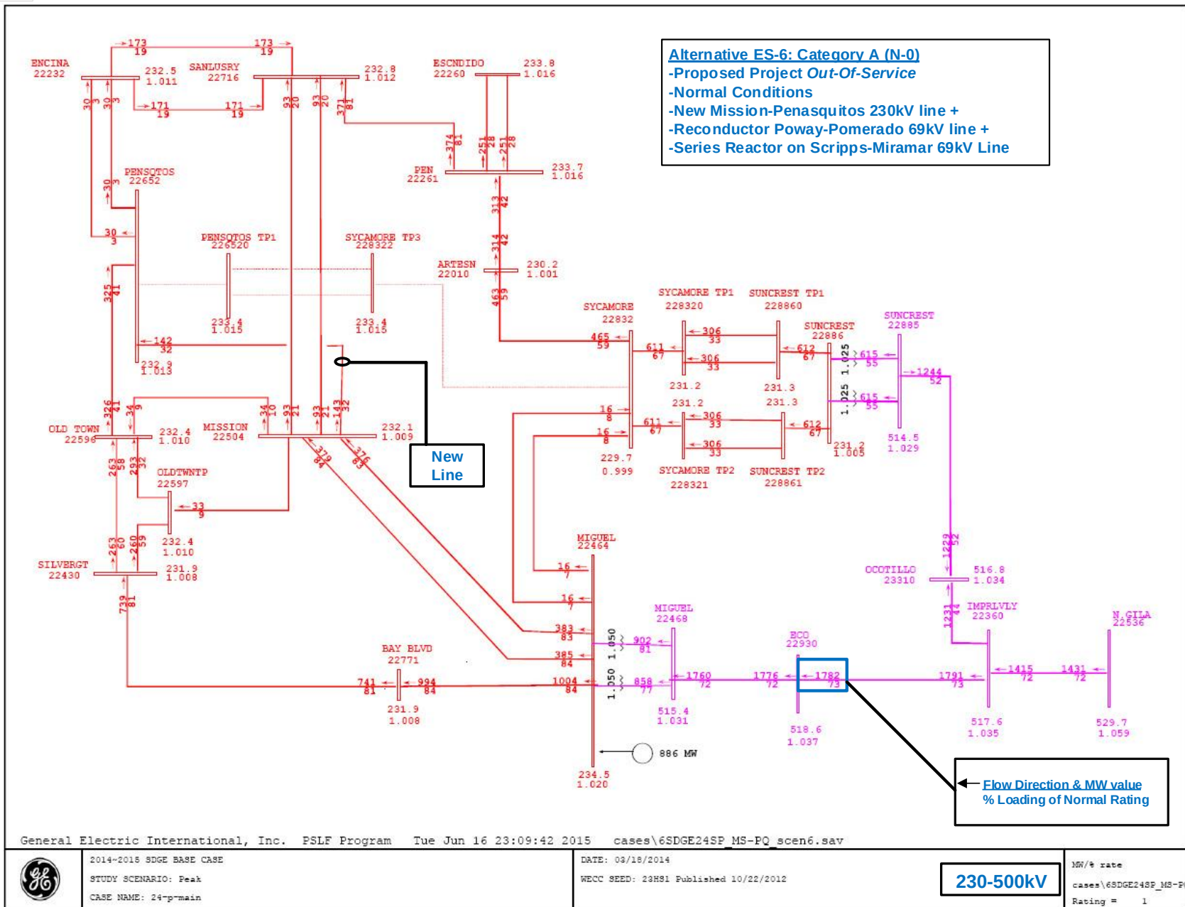
Figure 18 – ES-6, 230/500 kV Power Flow Plot, Normal condition
