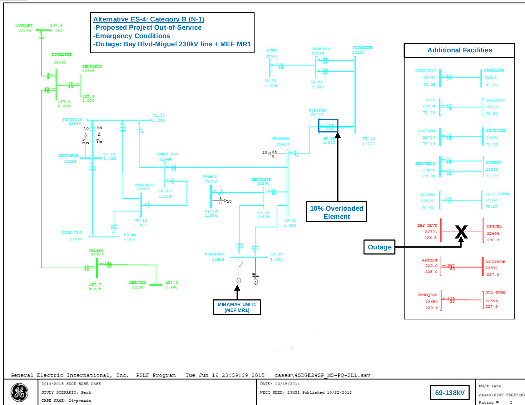
Figure 15 – ES-4, 69/138 kV Power Flow Plot, Single contingency
