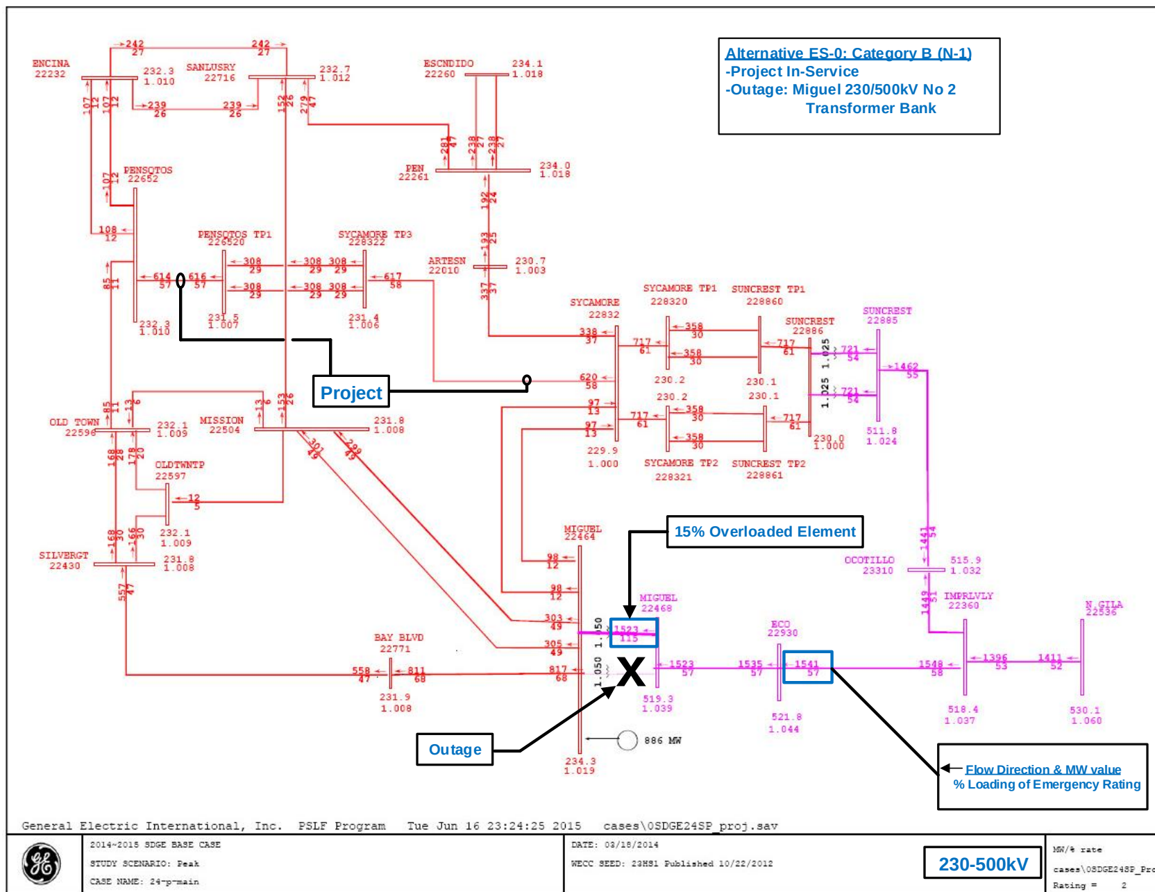
Figure 2 - ES-0, Power Flow Plot for Category B contingencies (230/500 kV System)
