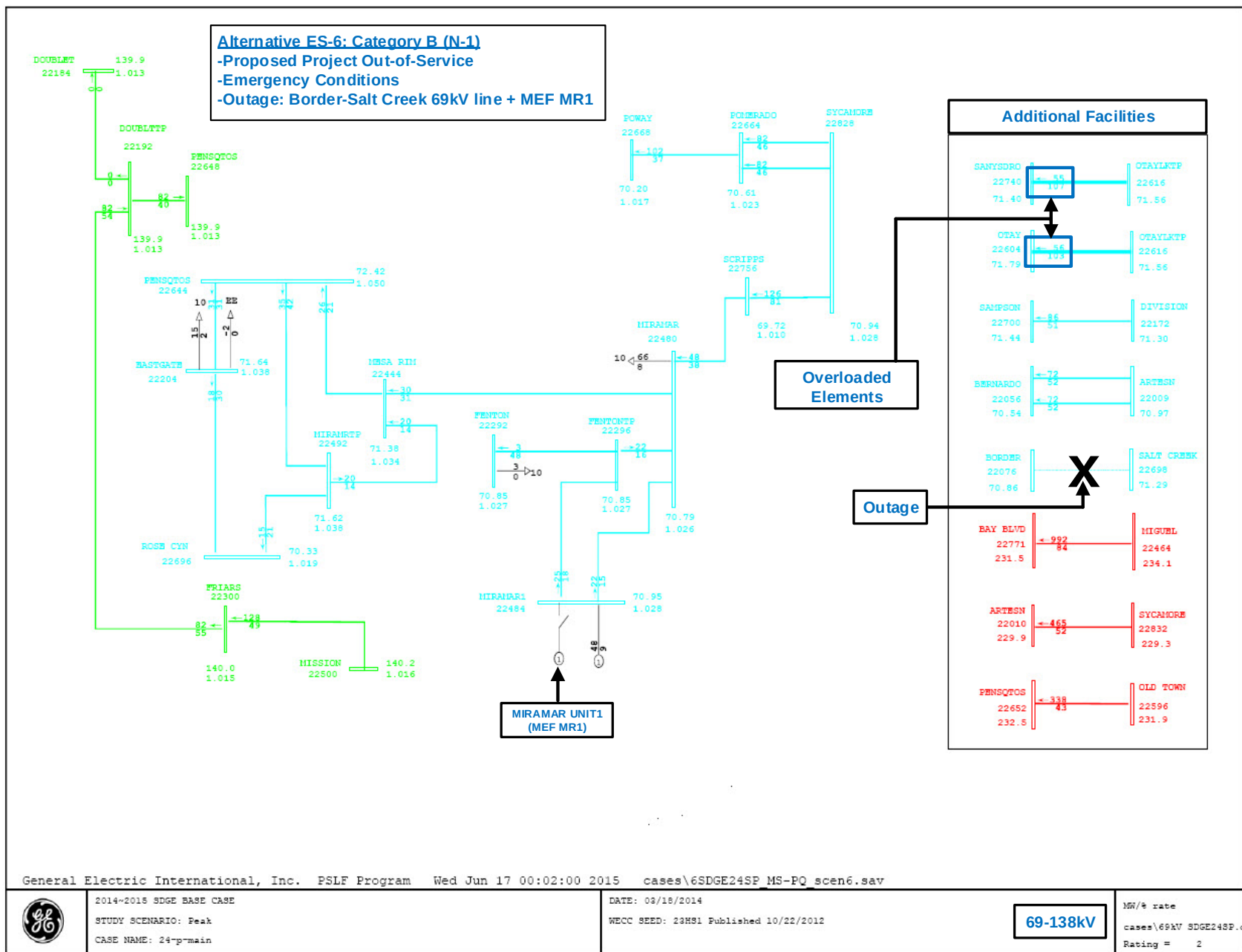
Figure 20 – ES-6, 69/138 kV Power Flow Plot, Single contingency
