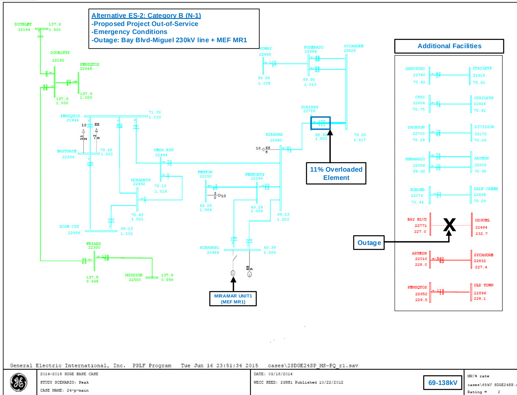
Figure 9 – ES-2, 69/138 kV Power Flow Plot, Single contingency
