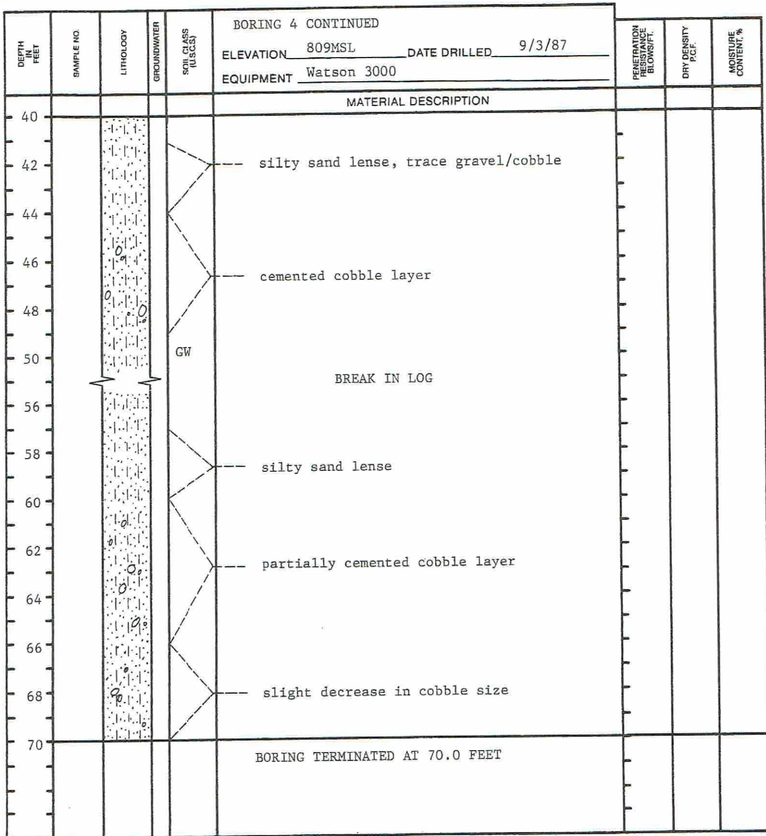
Figure A-7, Log of Test Boring 4 continued
