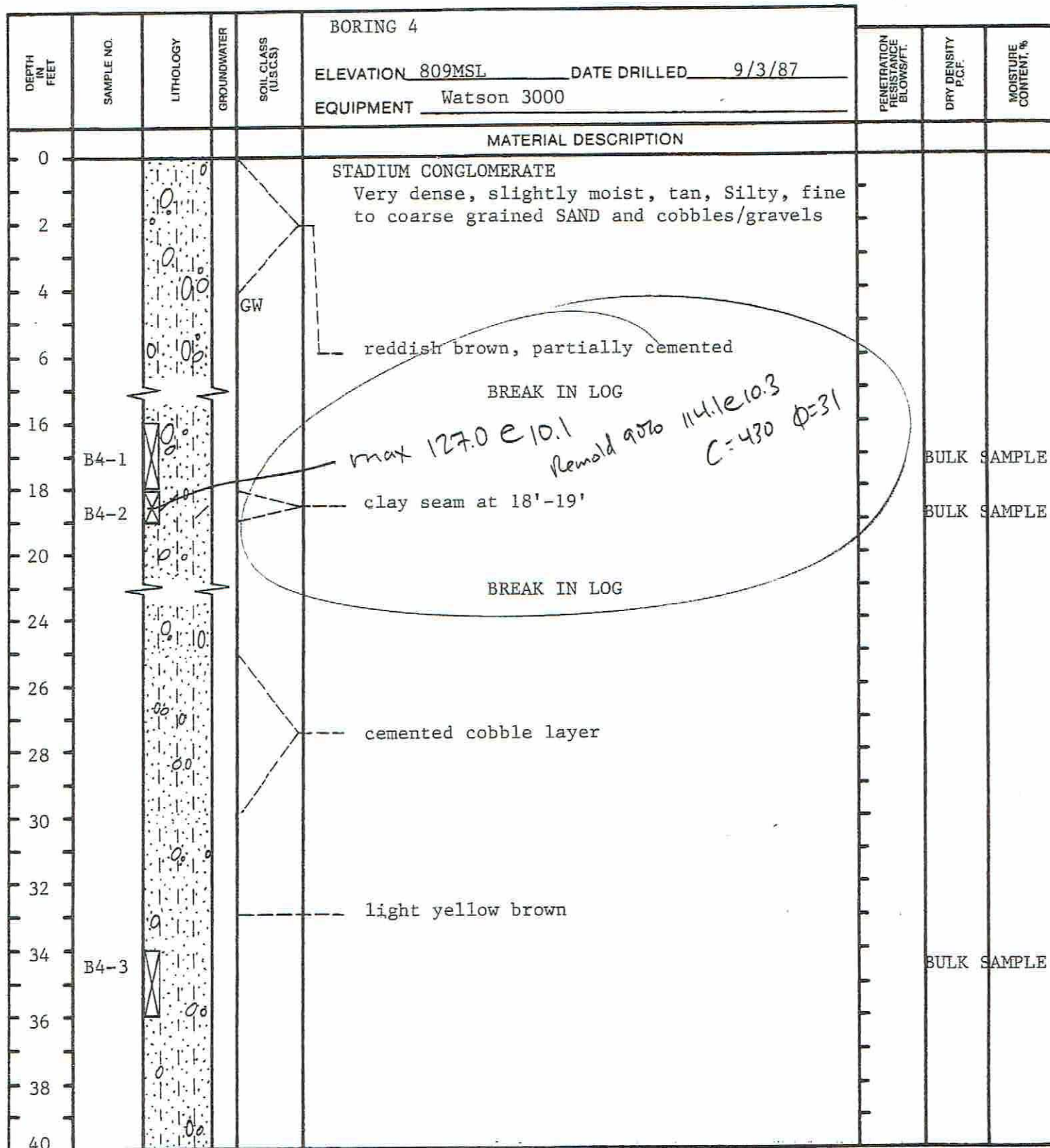
Figure A-6, Log of Test Boring 4
