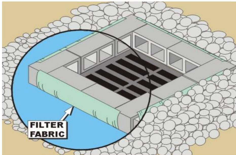
Block and gravel-type inlet protection.
