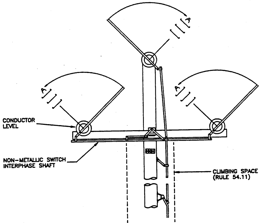
POLE TOP POSITION BRACKET CONSTRUCTION Fig. 58-2
