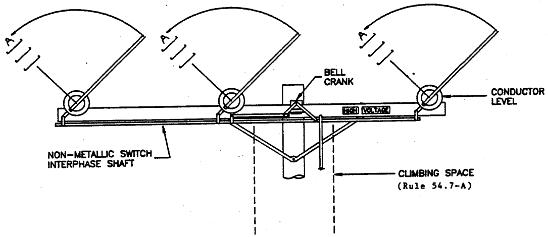
POLE TOP POSITION CROSSARM CONSTRUCTION Fig. 58-1
