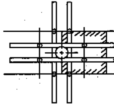
At Pole Top FIGURE 54-3
